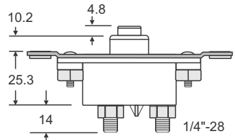
I9A-P21-N-xxx Automatic Reset TI
