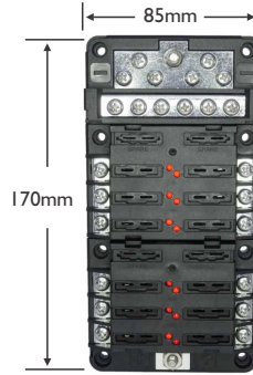
Height with cover 42mm
