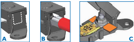
A Removable Top Wall B Input Cable Top Entry C Busbar Accessory No Cut-out Required
