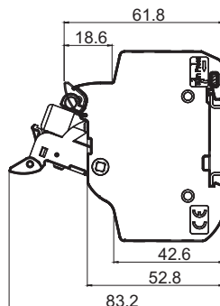
Single Pole
