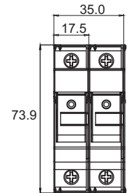
Double Pole
