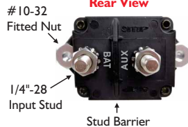
19A-P10 Series, Automatic Reset TI Non Indicating
