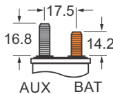
Terminal Specs 2 x #10-32 studs
