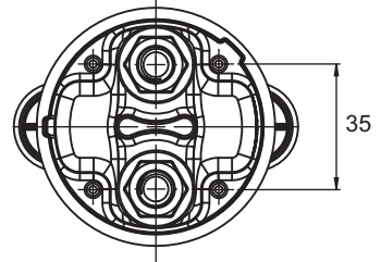
Bottom View 75940 (SPST)
