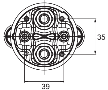
Bottom View 75930 (DPST)
