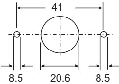
Mounting Diagram
