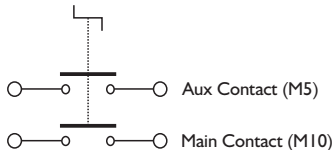
Electrical Diagram 75930 (DPST)
