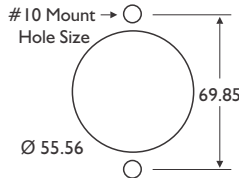
Recommended Panel Mounting Cut-Out
