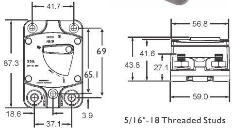
5/16" - 18 Threaded Studs
