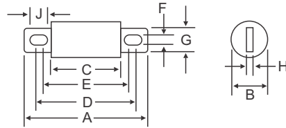
Diagram 1 (35A - 1200A)
