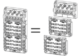
12 Way Fuse Base (with 12 Ground terminals)
