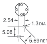
Recommended Mounting Pattern
