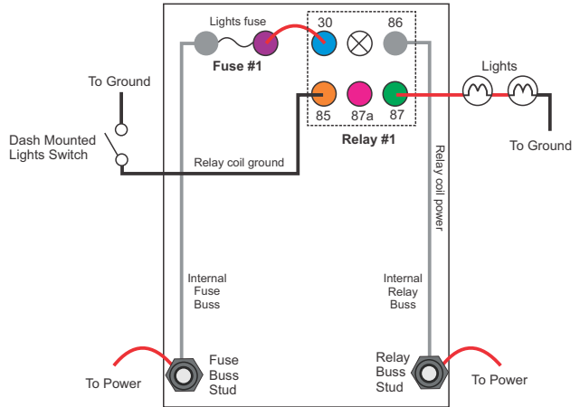
15305-2 Wiring Example (Bottom View).
