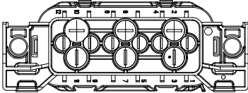
Terminal Numbering (Rear of Unit)
