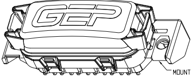
MOUNTING INSERT PDM-R3XXX M6 X 1.0
