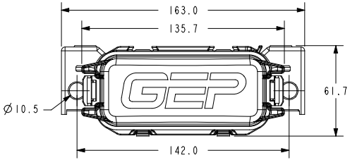
MOUNTING INSERT PDM-R3XXX M6 X 1.0
