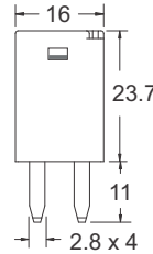
Dimensions in MM
