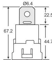
Skirted Relay with Removable Steel Bracket
