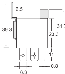
Clear Fuse Cover and Steel Bracket are Both Removable
