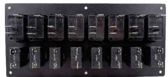
Loaded Rear View 8 Way Switch & Breaker Panel
