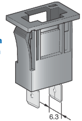
1/4" Q.C Terminals
