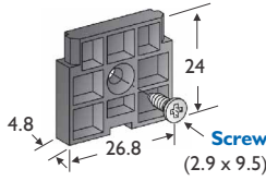
Fixing Plate
