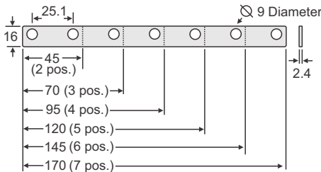
Midi Fuse (see p.24)
