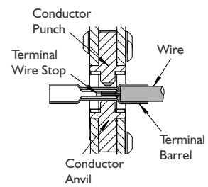
Crimping Butt Splice Connectors
