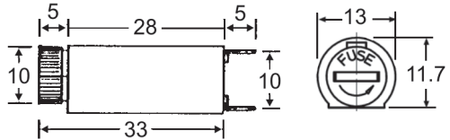
FH-PCV (Vertical Mount)
