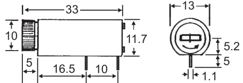
FH-PCO (Horizontal Mount)
